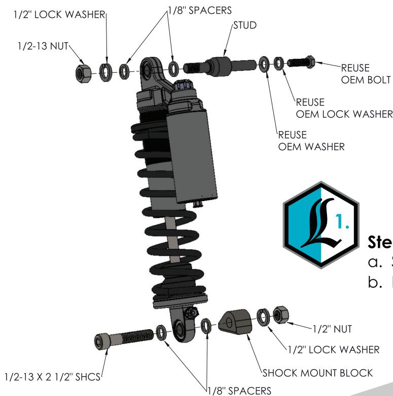
FIGURE A FXR LH SHOCK
