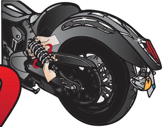
FIGURE C ADJUST SAG EQUALLY ON BOTH SIDES
